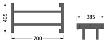
Optional back bracket & clip bracket
